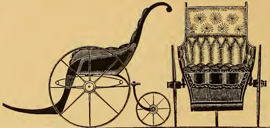
INVALID CHAIR.— \frac{1}{2} IN. SCALE.
